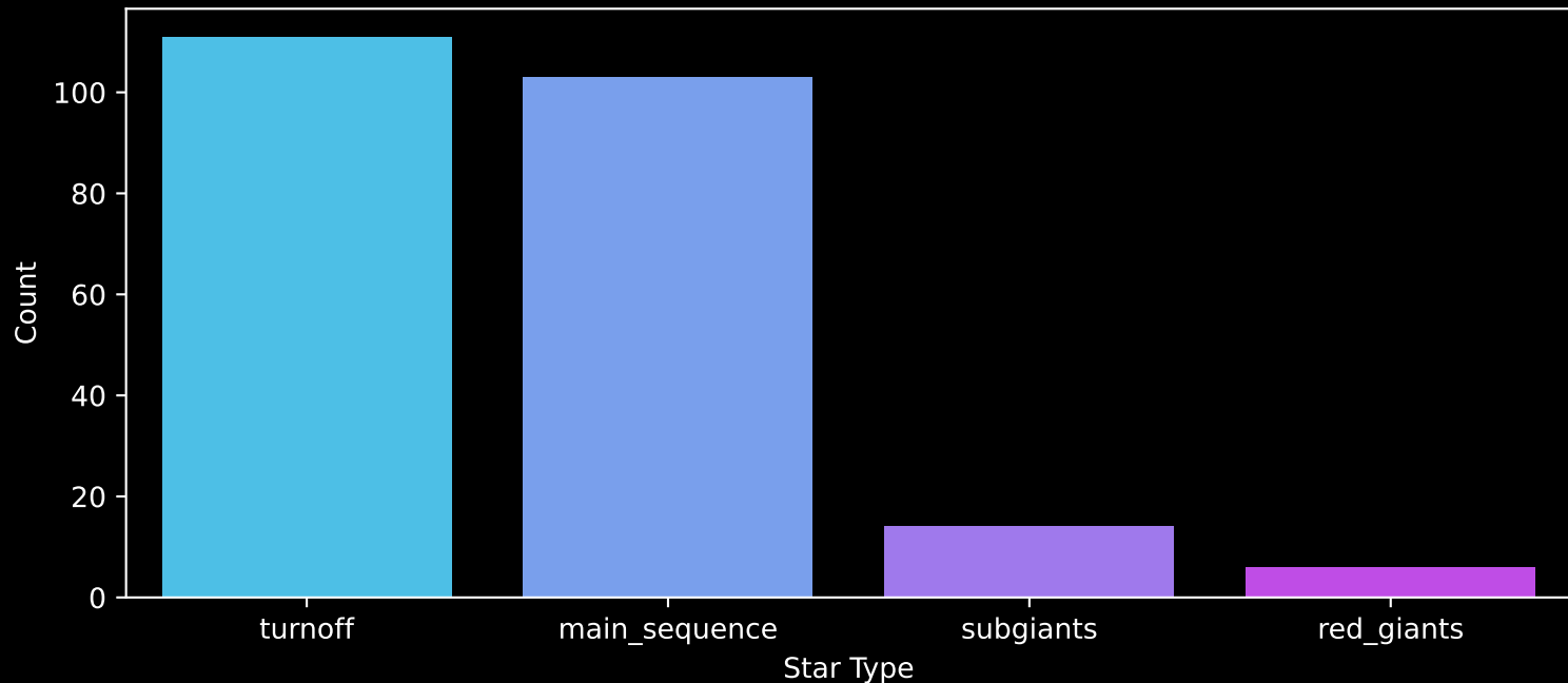
APOGEE DR17 Field: [CA_163-08_btx] Count plot of Star Type
