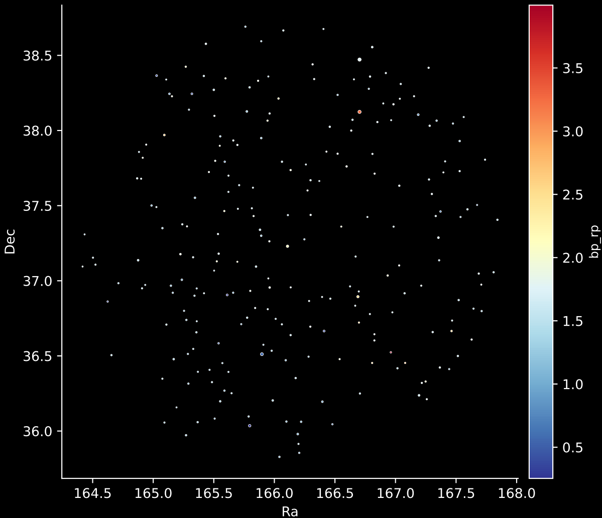
APOGEE DR17 Field: [CA_163-08_btx] Stars: 234
