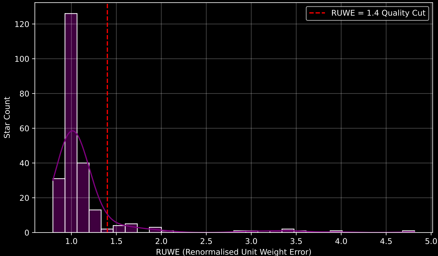
GAPOGEE DR17 Field [CA_163-08_btx] RUWE Distribution (n= 233)
