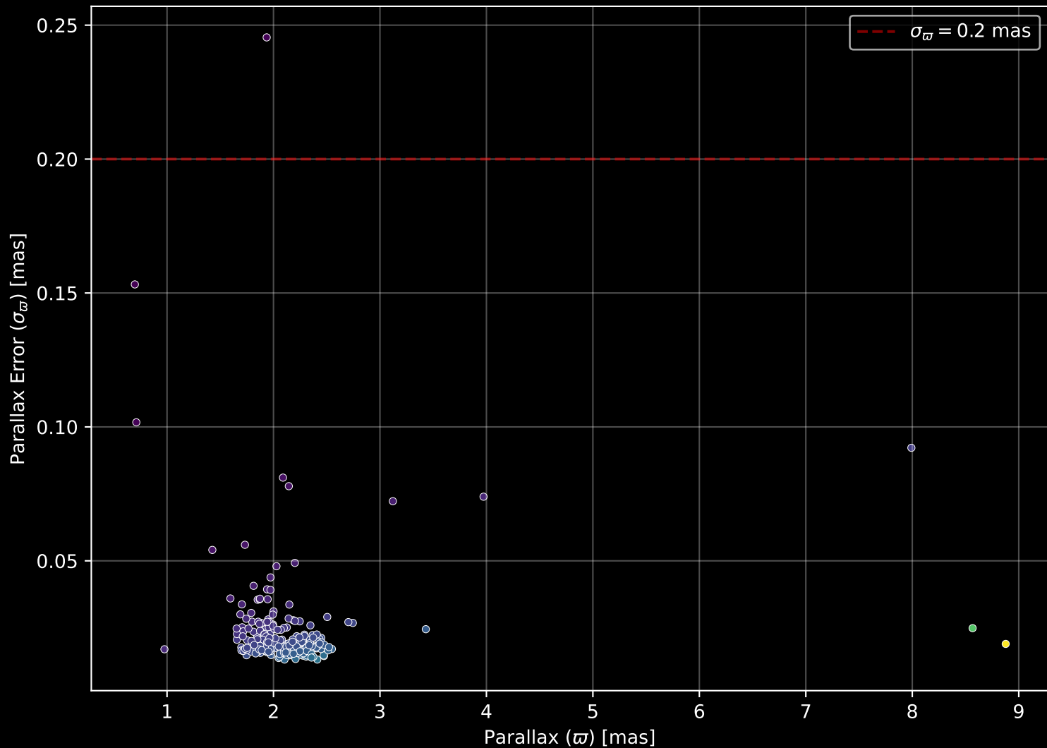
APOGEE DR17 Field: [CA_163-08_btx] Parallax Quality (n= 234)
