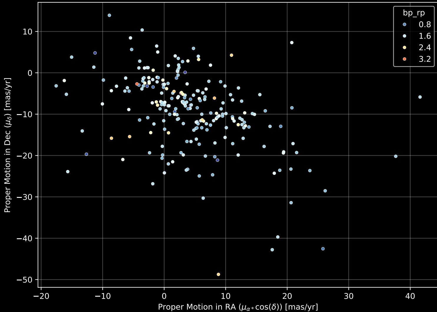
APOGEE DR17 Field: [CA_163-08_btx] Proper Motion Diagram (n= 234)
