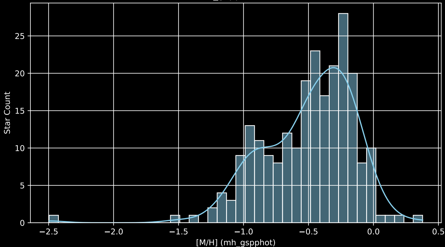
APOGEE DR17 Field: [CA_163-08_btx [M/H] (mh_gspphot) (n= 234)
